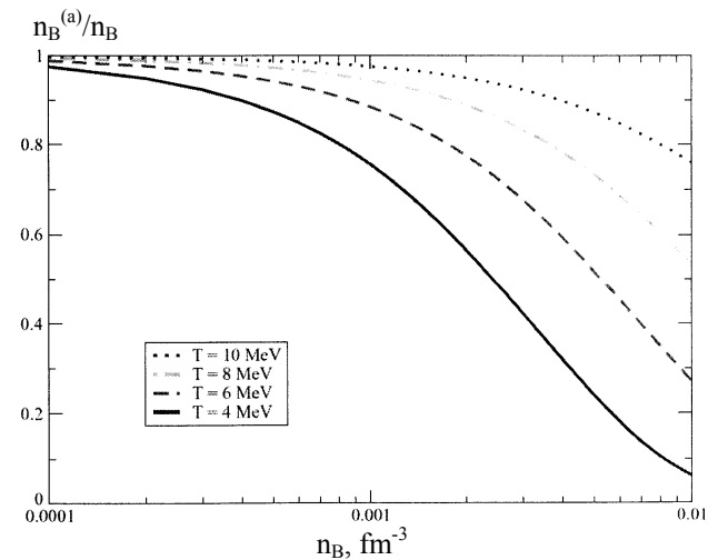
Fig. 2. The ratio between the ACCR baryon density n_B^{(a)} (no medium effects) and n (including medium effects) as a function of the baryon density n_B = n_p + n_n for various values of T (taken from Ref. [9]).
