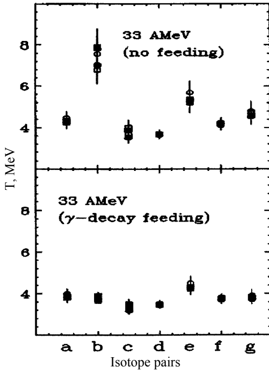
Fig. 1. Temperature extracted from double ratios of: a - ^4\text{He}/^3\text{He} , ^7\text{Li}/^6\text{Li} ; b - ^4\text{He}/^3\text{He} , ^{10}\text{Be}/^9\text{Be} ; c - ^4\text{He}/^3\text{He} , ^{11}\text{B}/^{10}\text{B} ; d - ^4\text{He}/^3\text{He} , ^{13}\text{C}/^{12}\text{C} ; e - ^7\text{Li}/^6\text{Li} , ^{12}\text{C}/^{11}\text{C} ; f - ^{12}\text{C}/^{11}\text{C} , ^{13}\text{C}/^{12}\text{C} ; g - ^7\text{Be}/^6\text{Li} , ^{12}\text{C}/^{11}\text{B} yield ratios for the reactions ^{40}\text{Ca} + ^{58}\text{Ni} (filled circles), ^{40}\text{Ar} + ^{58}\text{Ni} (open circles), ^{40}\text{Ca} + ^{58}\text{Fe} (filled squares), and ^{40}\text{Ar} + ^{58}\text{Fe} (open squares) at beam energies of 33 MeV/nucleon before (top) and after (bottom) accounting for populations of \gamma -decaying states (taken from Ref [8]).
