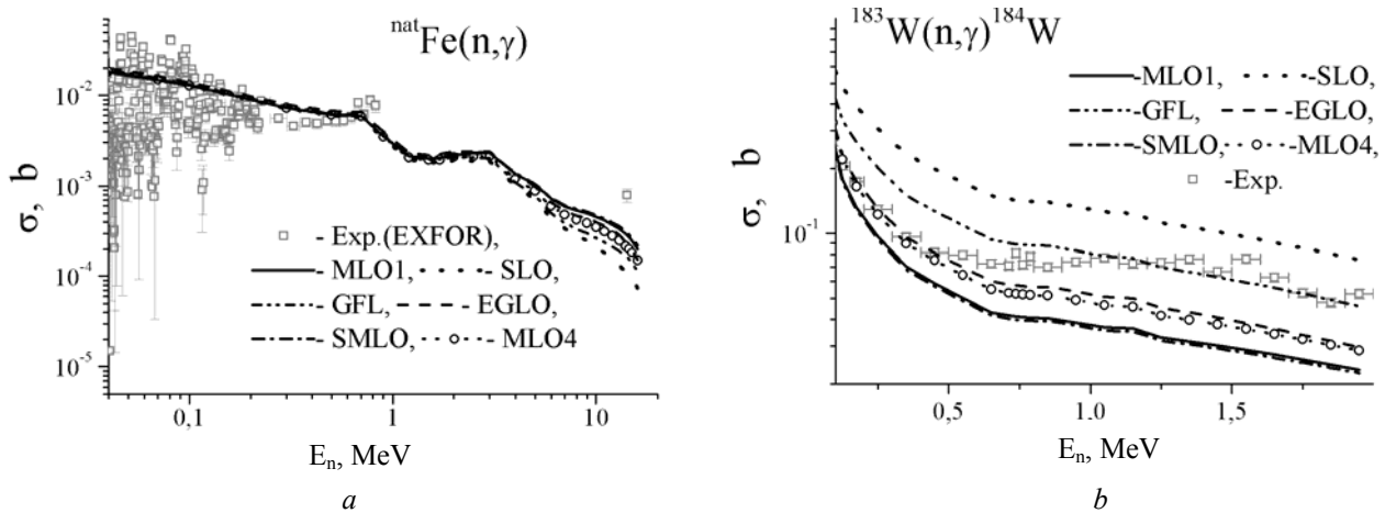
Fig. 6. The excitation function of ^{nat}\text{Fe}(n, \gamma) and ^{183}\text{W}(n, \gamma)^{184}\text{W} reactions using different RSF models. Experimental data are taken from EXFOR data library for panel a and [12] for panel b.
