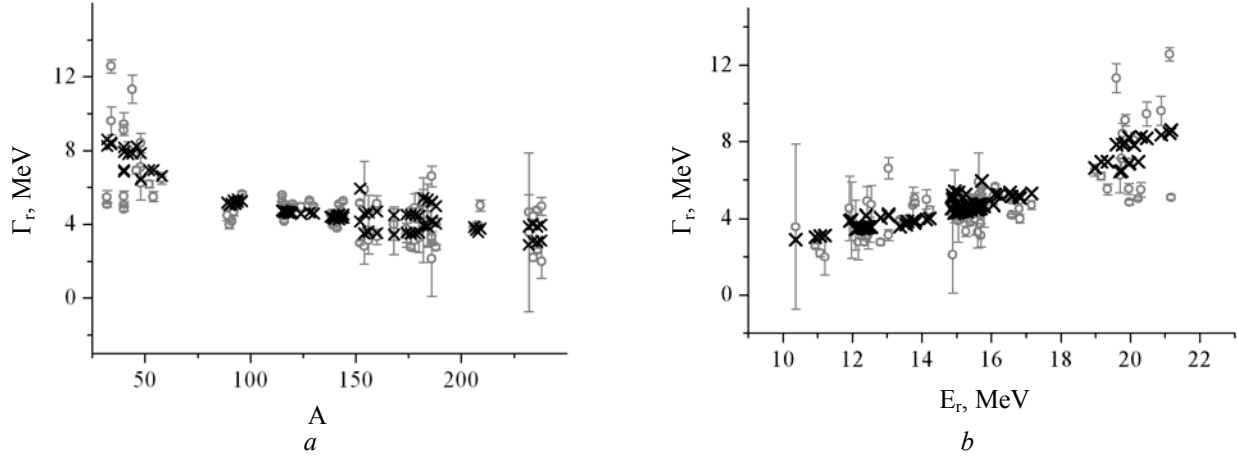
Fig. 1. Mean GDR widths as a function of mass number ( a ) and GDR energies ( b ) calculated by the use of SLO model: open circles - renewed GDR parameters [3]; crosses - parameters obtained by the systematic (1).
