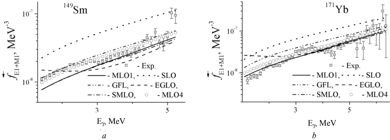
Fig. 4. The gamma-decay strength functions within different RSF models for ^{149}\text{Sm} (a) and for ^{171}\text{Yb} (b). Experimental data are taken from [8, 9].
